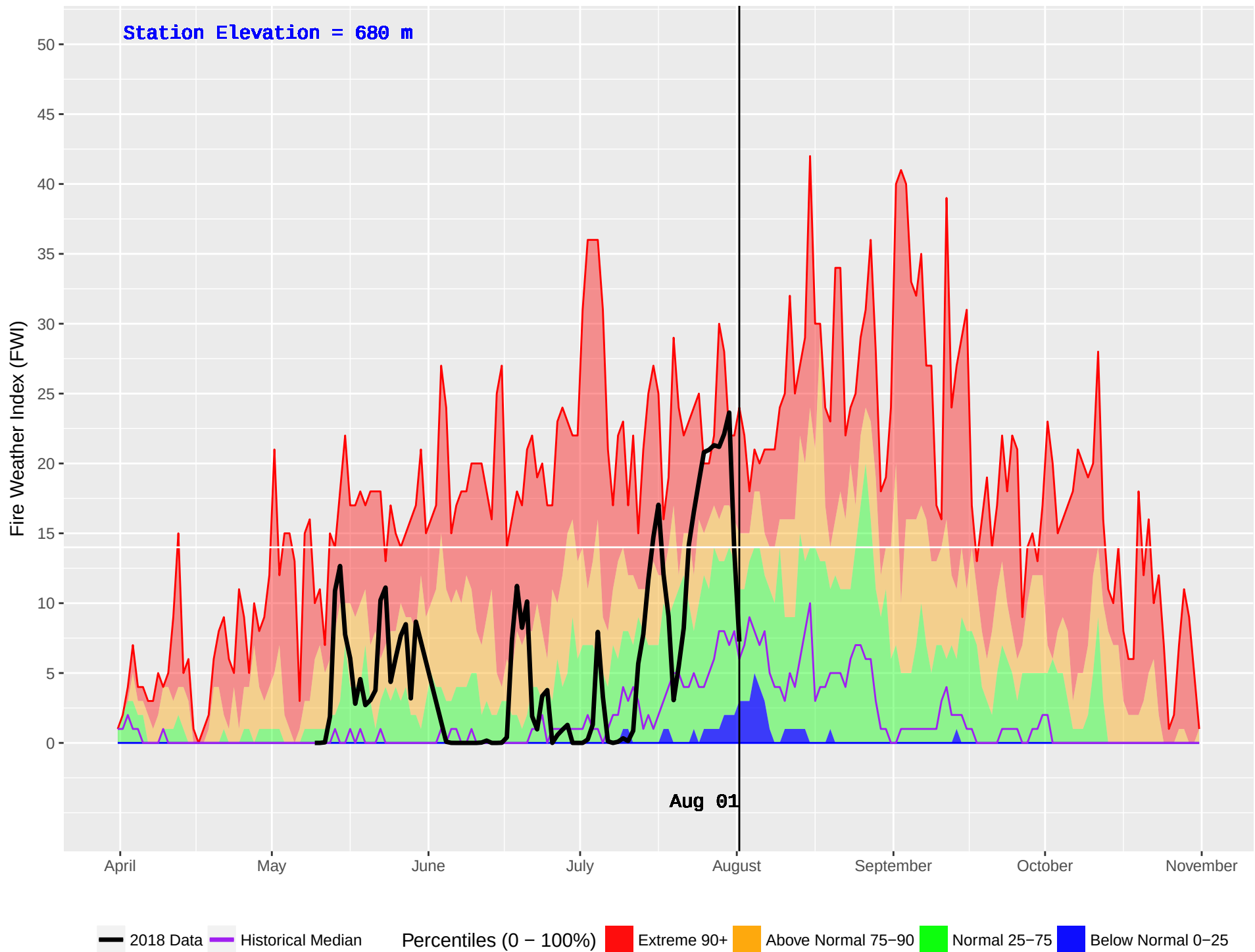
SUMMIT (11) : Historical (1985–2016) and Current (2018) Daily Fire Weather Index (FWI)
