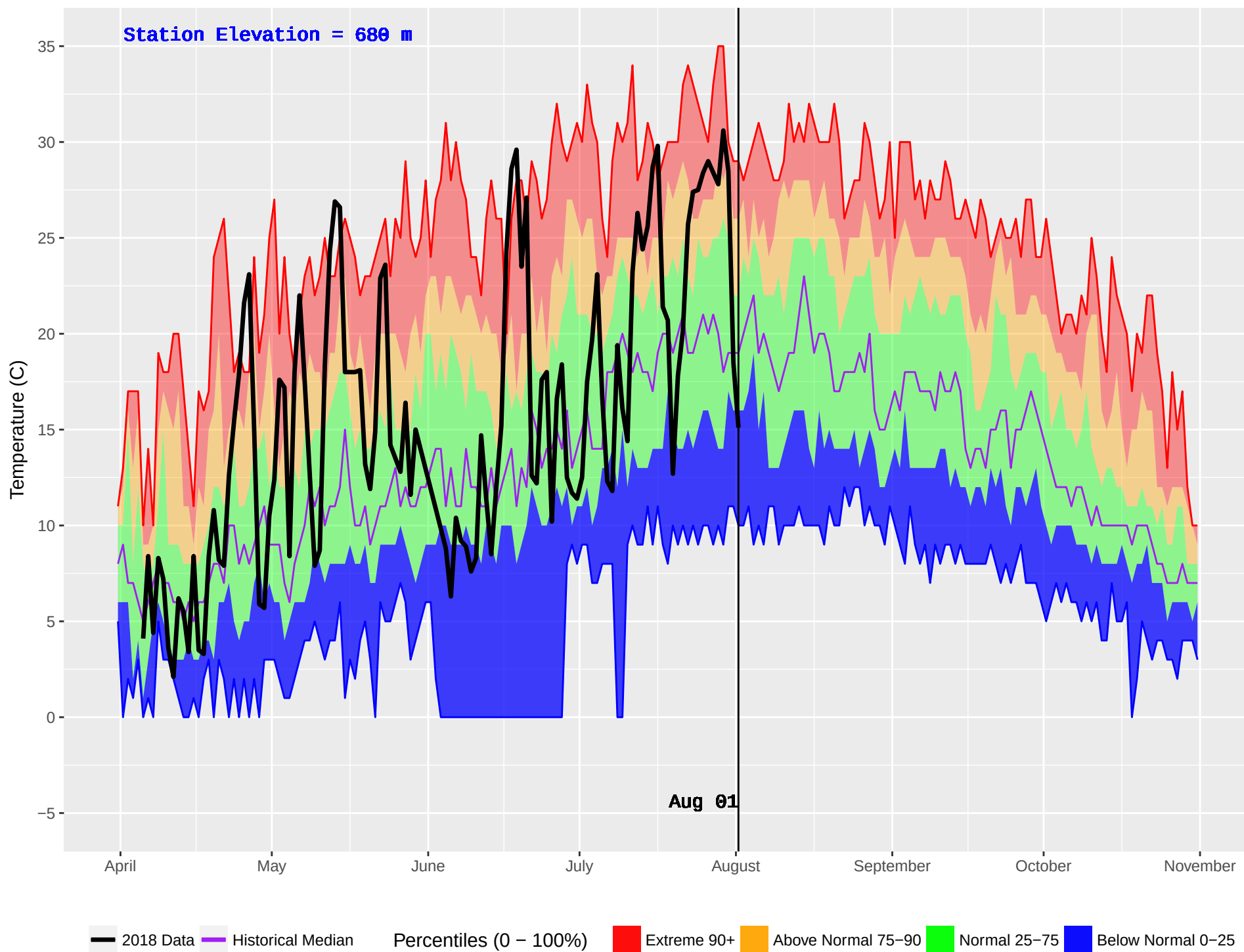
SUMMIT (11) : Historical (1985–2016) and Current (2018) Daily Temperature
